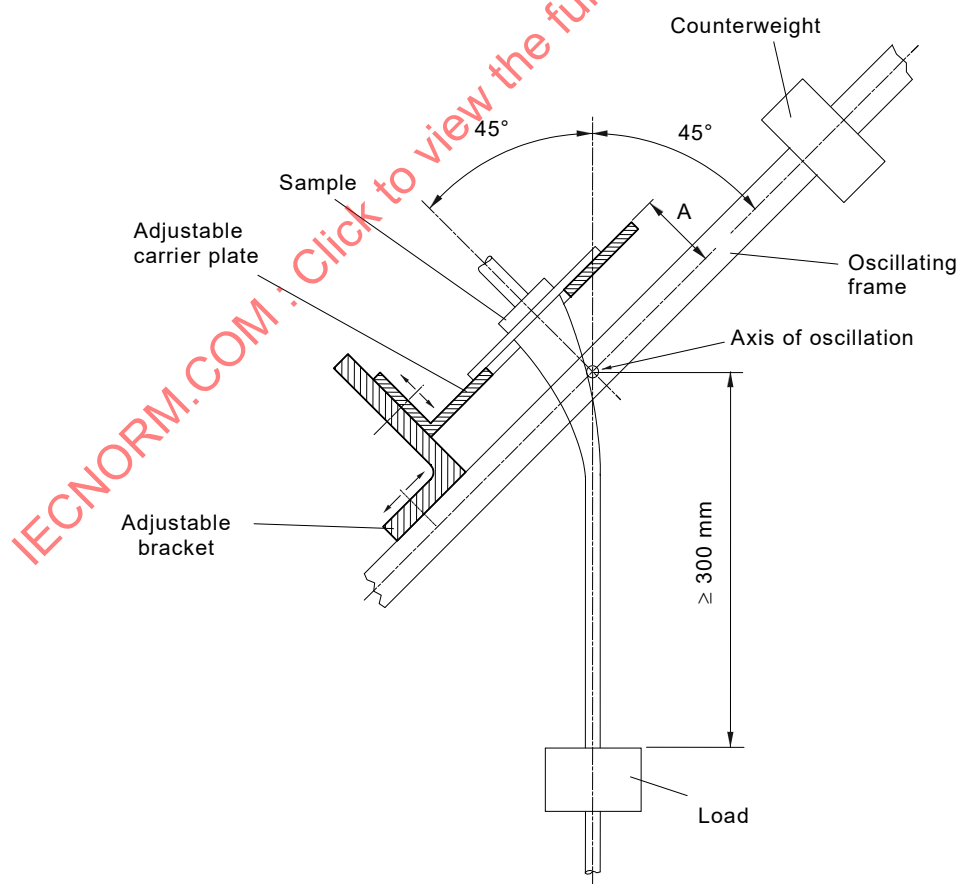
Figure 12 – Flexing test apparatus
