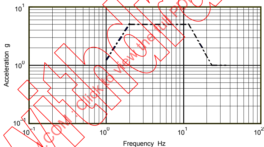
Figure 5 – Seismic synthesized waveform B
