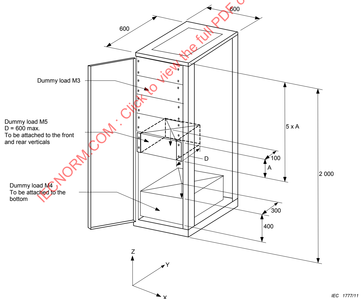
Figure 1 – Cabinets or racks configuration for test set up
