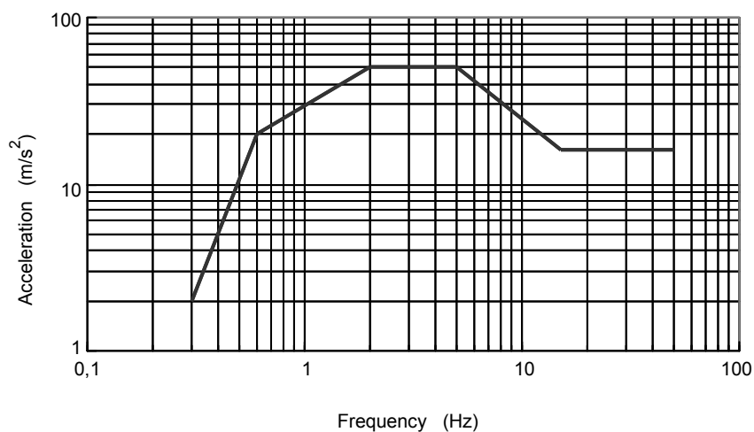
Figure 3 – The RRS for test wave (damping ratio 2%)
