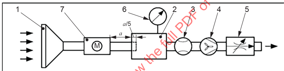
b) Setup for CFE without duct
