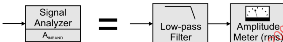
Figure 3 – In-band amplitude
