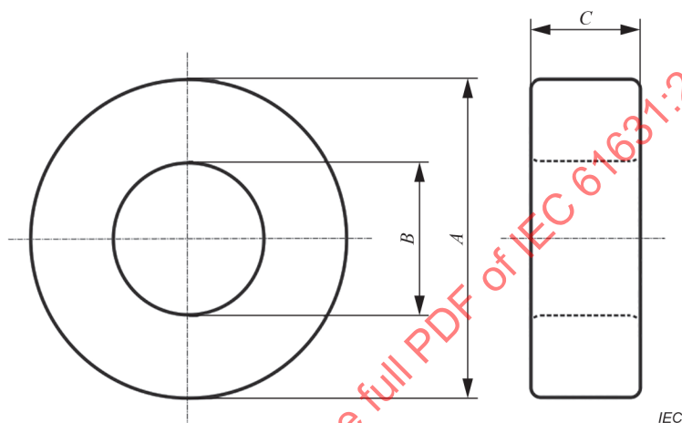
Figure B.1 – Dimensions of ring-core
