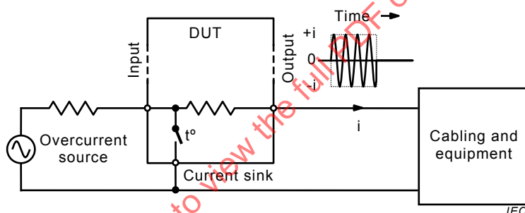
Figure B.3 – Thermally operated (heat coil) three-terminal shunt current limiter
