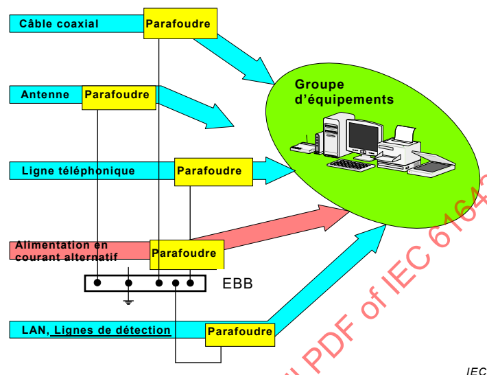
Figure 10 – Parafoudres individuels
