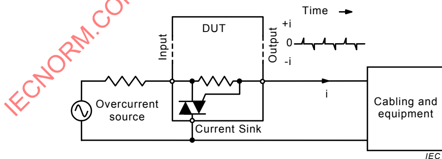
Figure B.7 – Electronic (gated bidirectional thyristor) three-terminal shunt current limiting component
