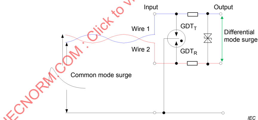
Figure F.4 – SPD circuit with inter-wire protection to limit the differential surge
