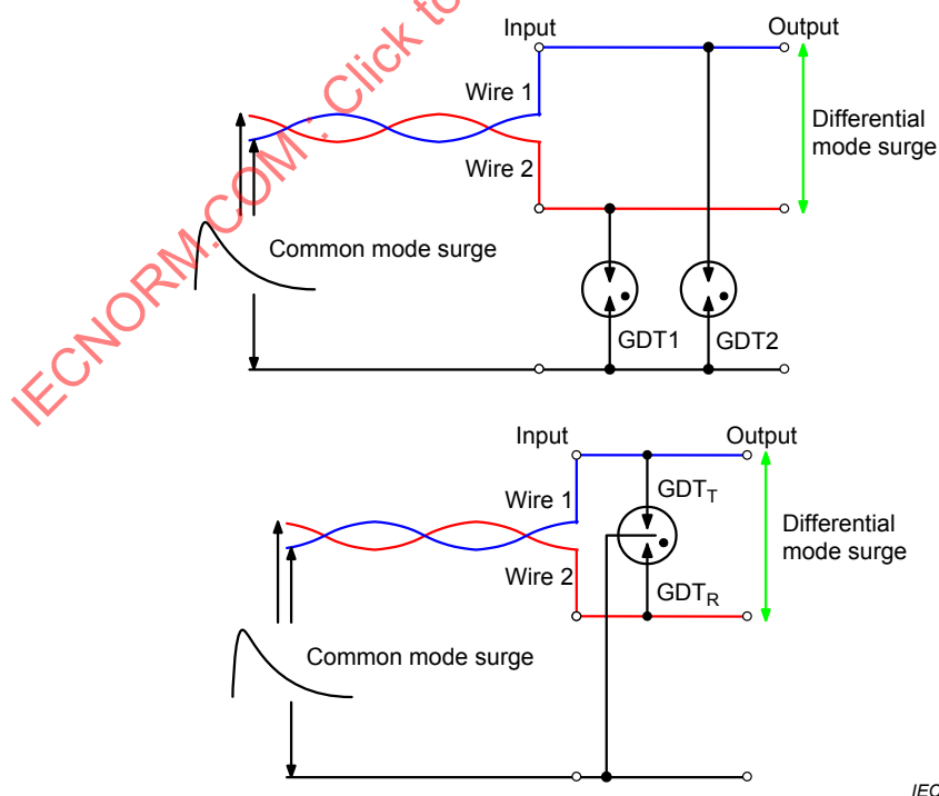
Figure F.2 – Common mode to differential mode surge conversion by asynchronous SPD operation
