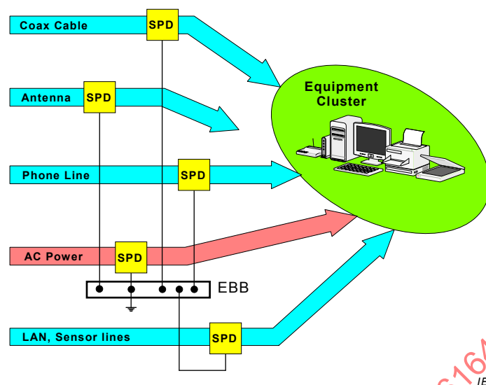
Figure 10 – Individual SPDs
