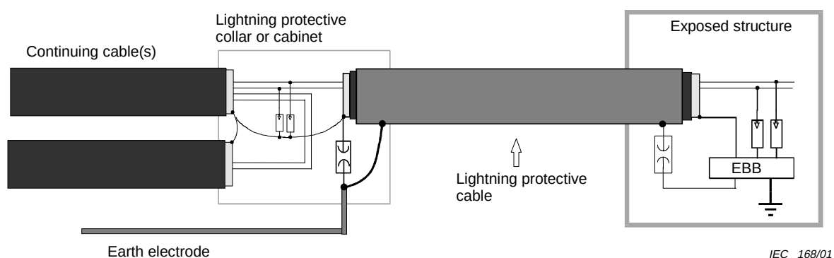
Figure 7b – Shielded cable
