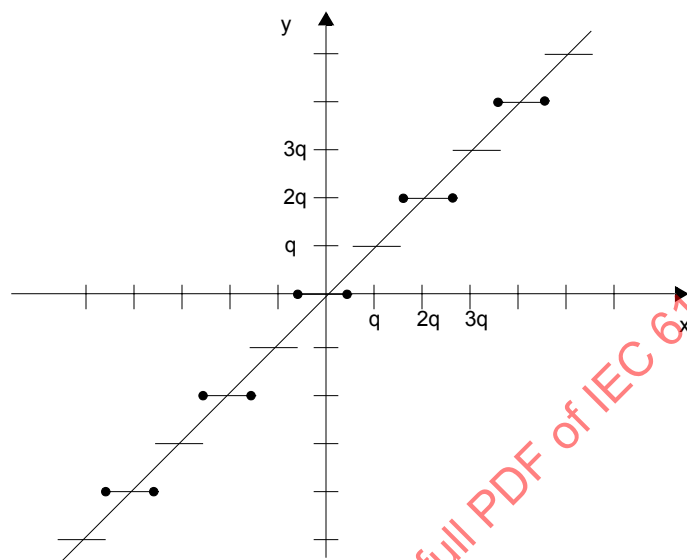
Figure 12—Convergent rounding
