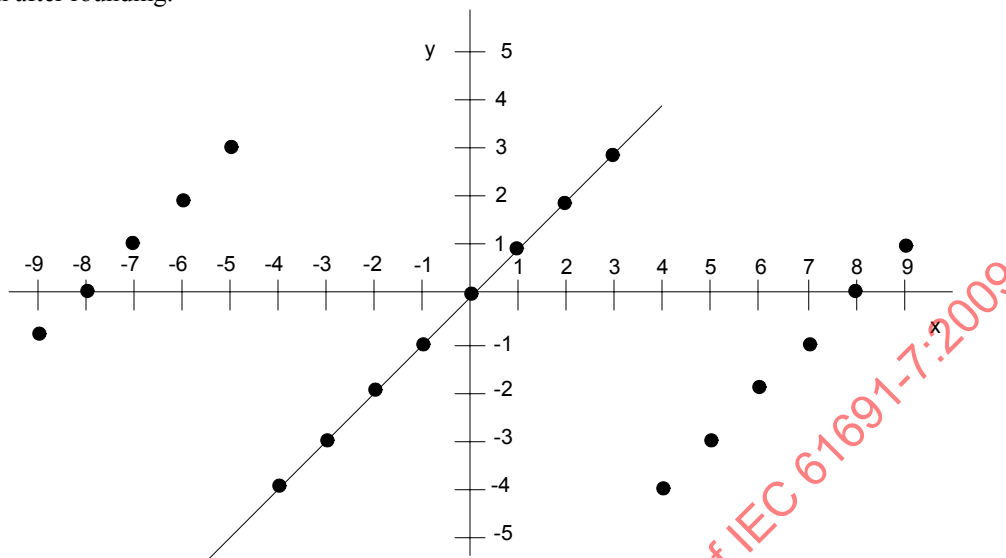
Figure 4—Wrap-around with n\_bits = 0 for signed numbers
