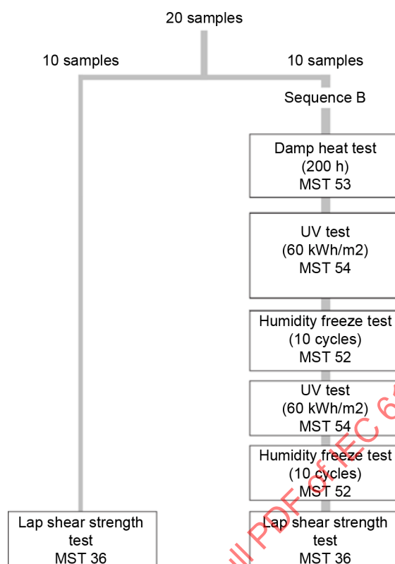
Figure 15 – Lap-shear test flow
