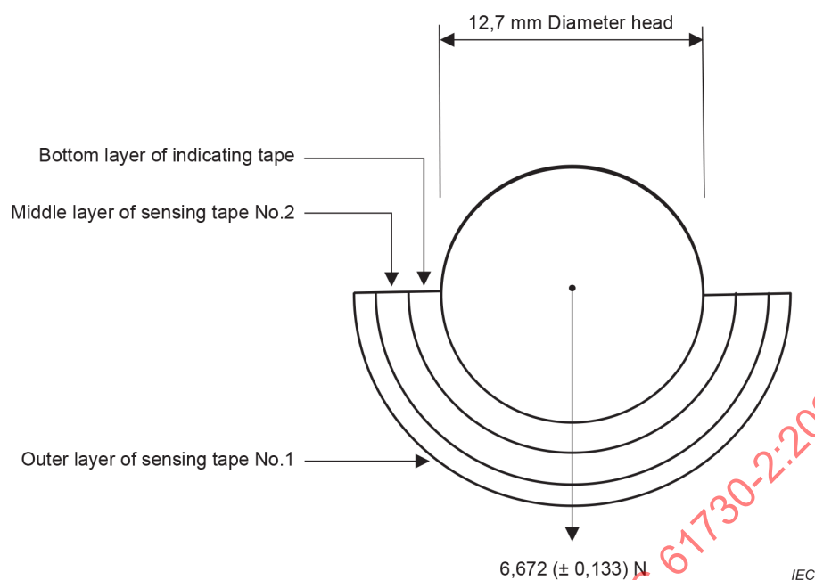
Figure 3 – Test apparatus MST 06
