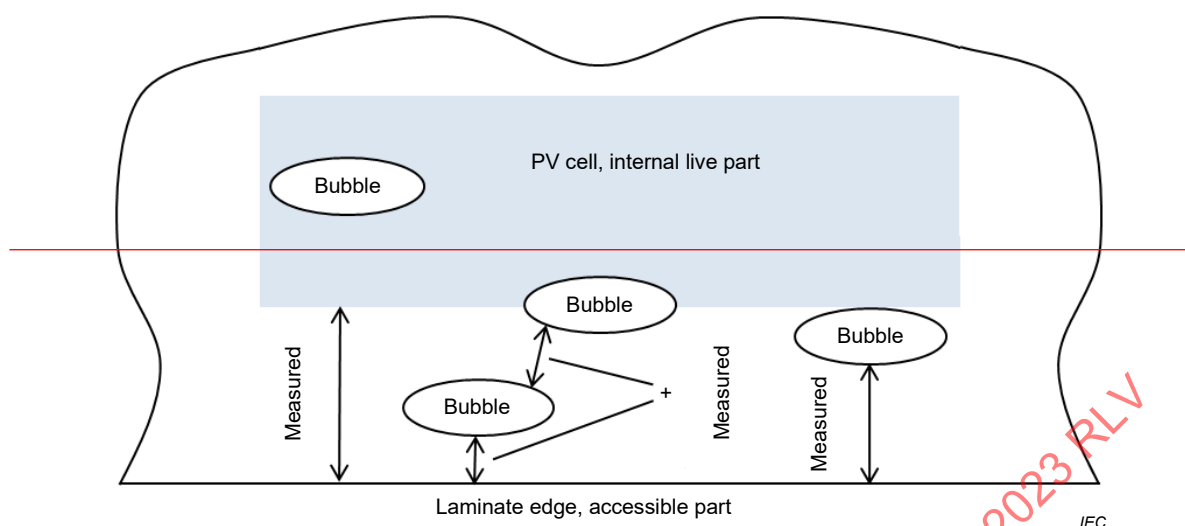
Figure 2a – Example for delamination assessment when measuring creepage or distance through insulation
