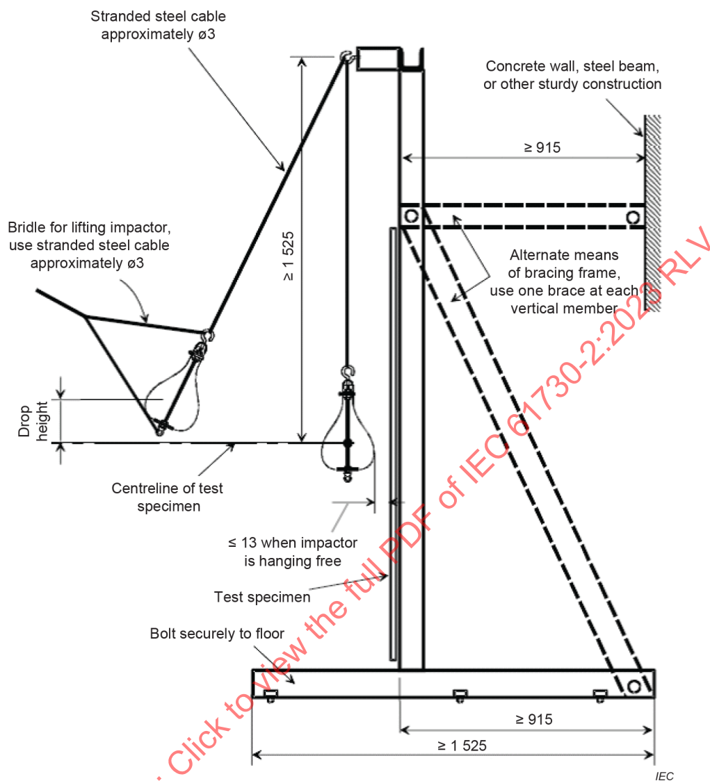
Figure 9 – Impact test frame 1
