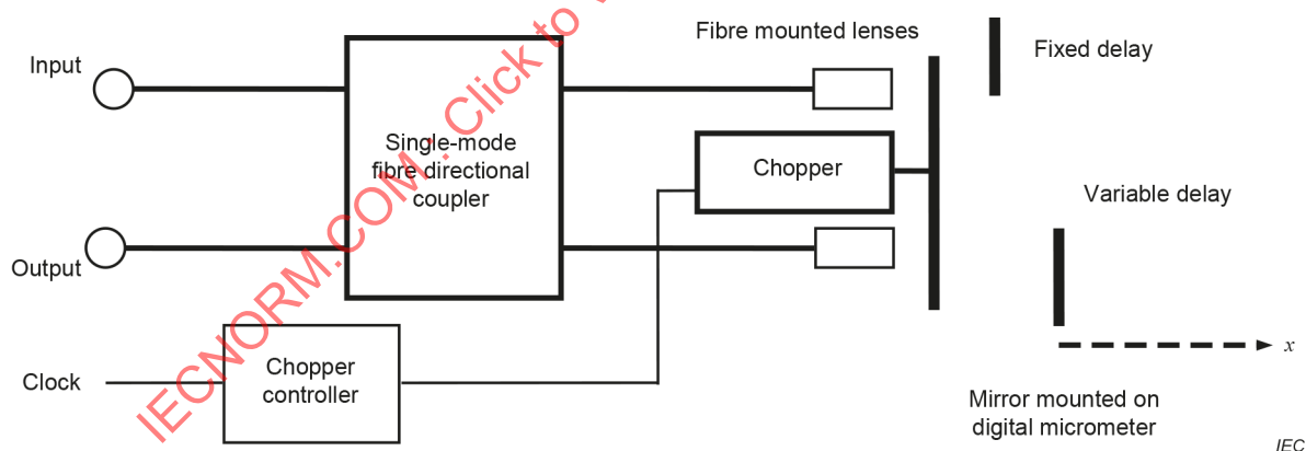
Figure 3 – Typical differential delay (dispersion) simulator for CD test set calibration
