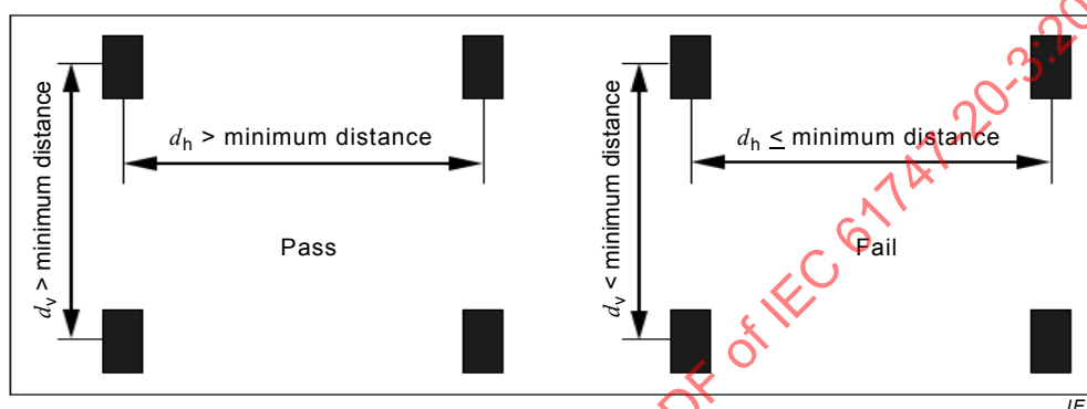
Figure 4 a) – Bright subpixel defect to bright subpixel defect
