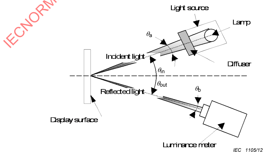
Figure 5 – Example of standard set-up for specular reflection measurements
