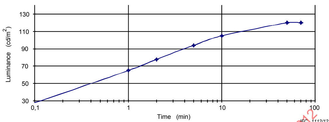
Figure 12 – Example of warm-up characteristic
