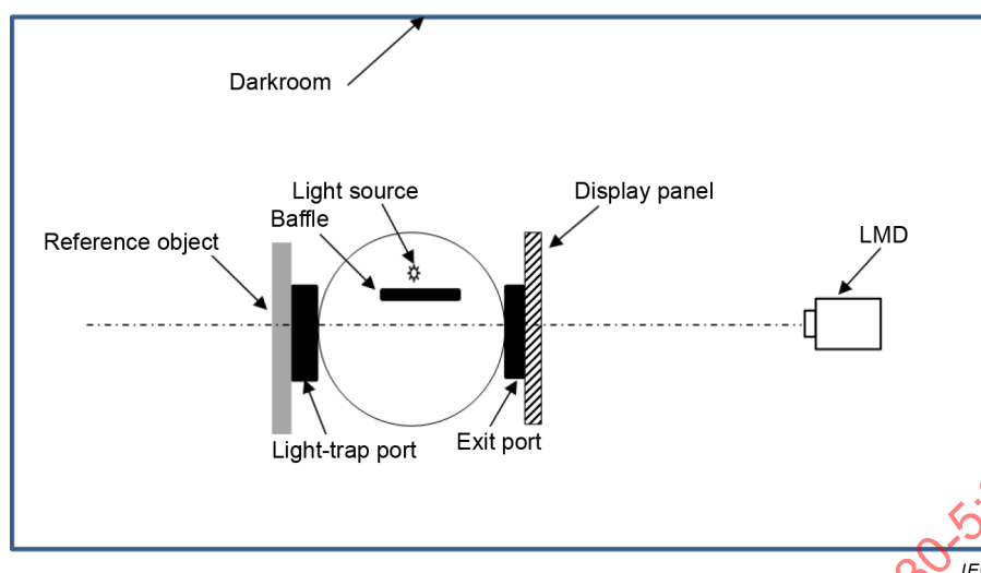
Figure 5 – Measurement system and its configuration
