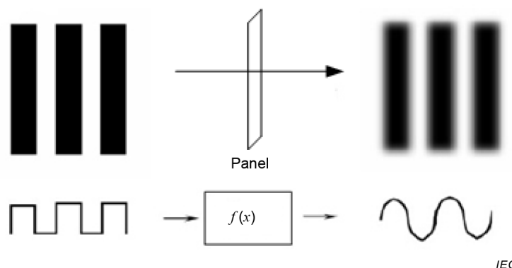
Figure 8 – Luminance curve of reference object
