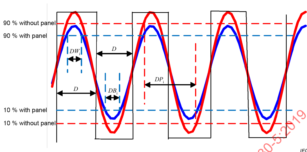
Figure 9 – Definition of test parameters
