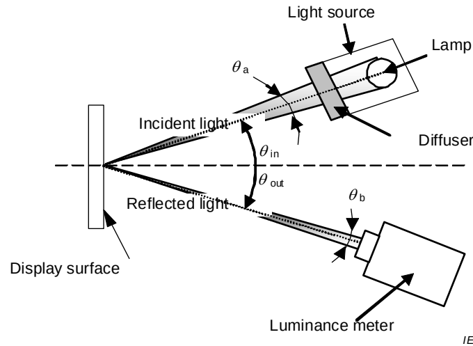
Figure 17 – Example of standard set-up for specular reflection measurements
