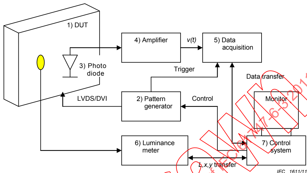
Figure 7 – Set-up to measure the temporal step response
