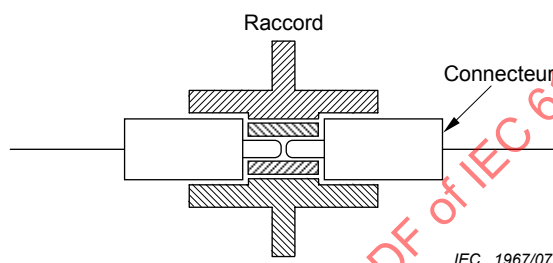
Figure 1 – Assemblage de fibres-amorces
