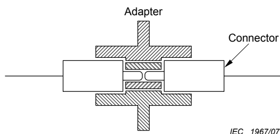
Figure 1 – Pigtail assembly
