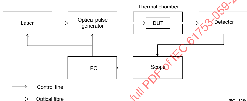
Figure G.2 – Response time testing set-up
