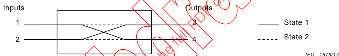
Figure 2 – Configuration of 2 × 2 spatial switch, non-crossover type
