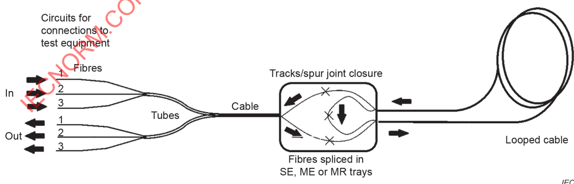
Figure A.1 – Track/spur joint configuration sample
