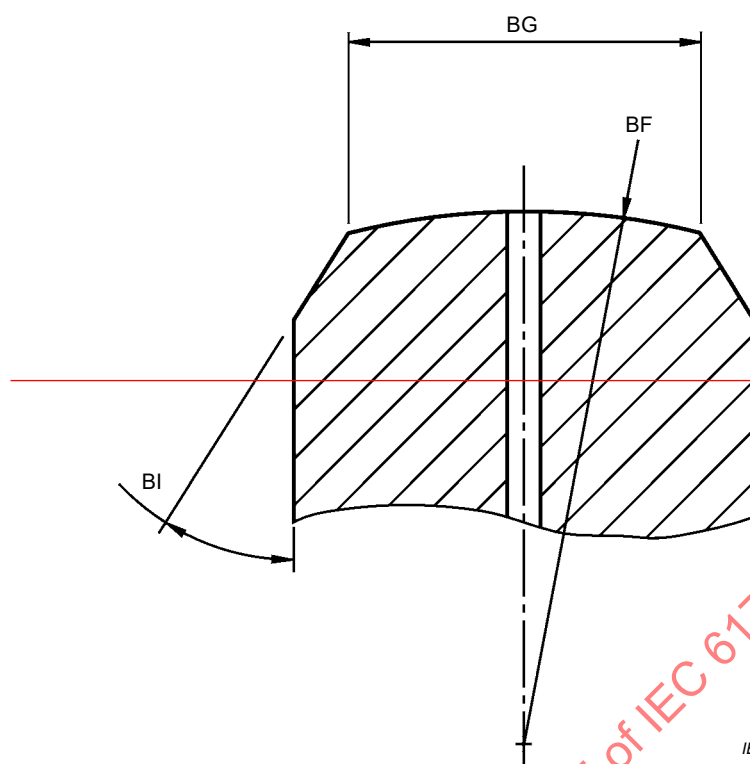
Figure 2 — Plug connector interface — Expanded view A (see Tables 1 and 2 for dimensions)
