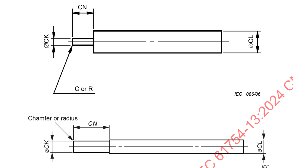
Figure 5 – Pin gauge for active device receptacle
