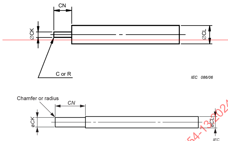
Figure 3 – Pin gauge for adaptor
