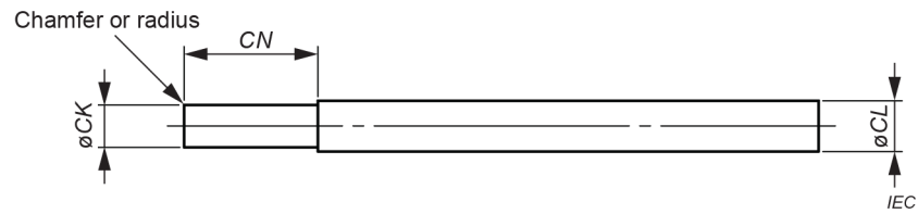
Figure 5 – Pin gauge for active device receptacle
