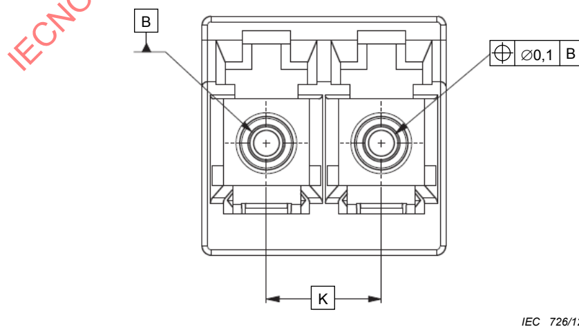
Figure 8 – Duplex active device receptacle interface
