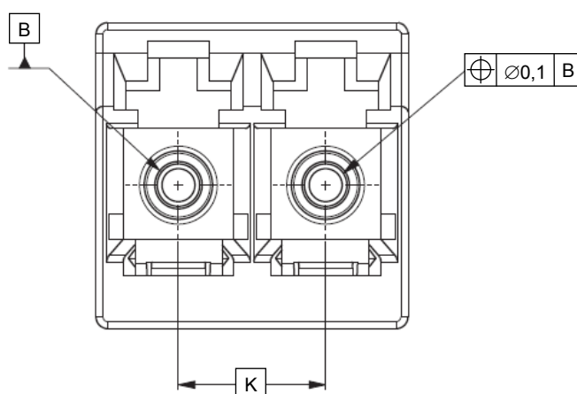
Figure 5 – Interface de raccords duplex
