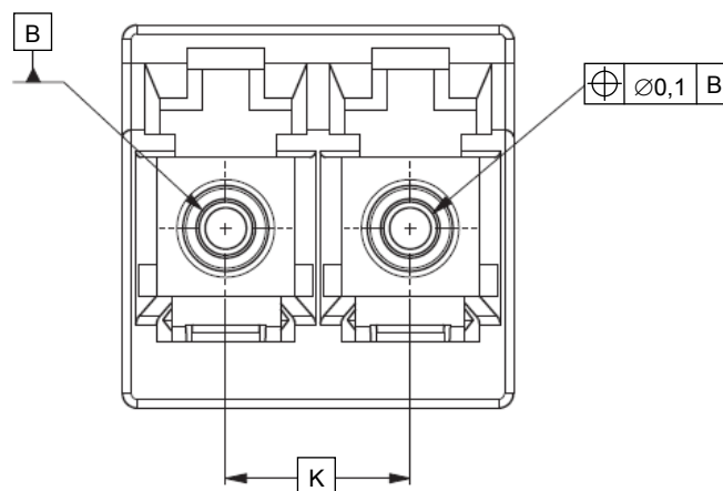
Figure 5 – Duplex adaptor interface
