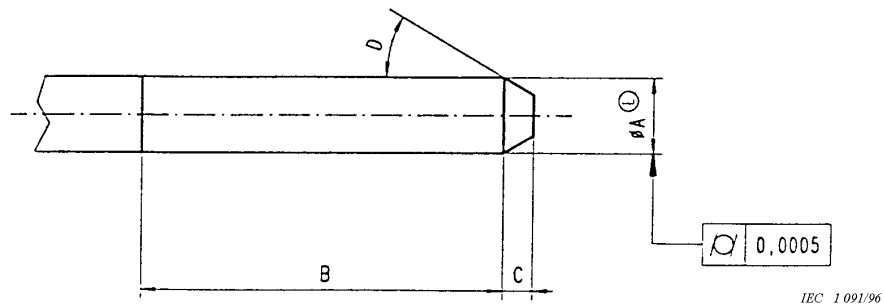
Figure 4 – Gauge pin for resilient alignment sleeve
