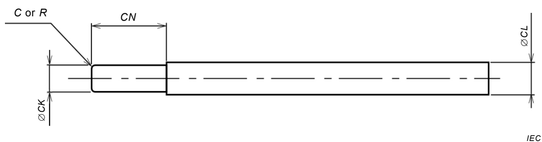
Figure 2 – Pin gauge for adaptor
