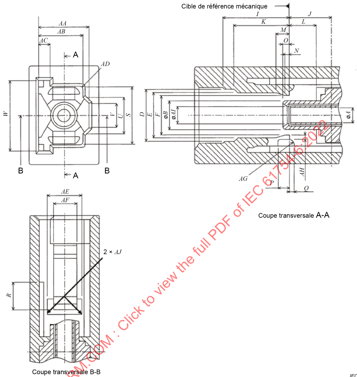
Figure 3 – Interface de raccord simplex – Pousser/tirer
