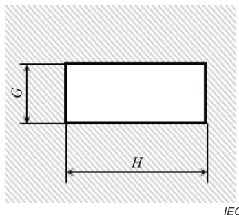
Figure D.4 – Panel cut out
