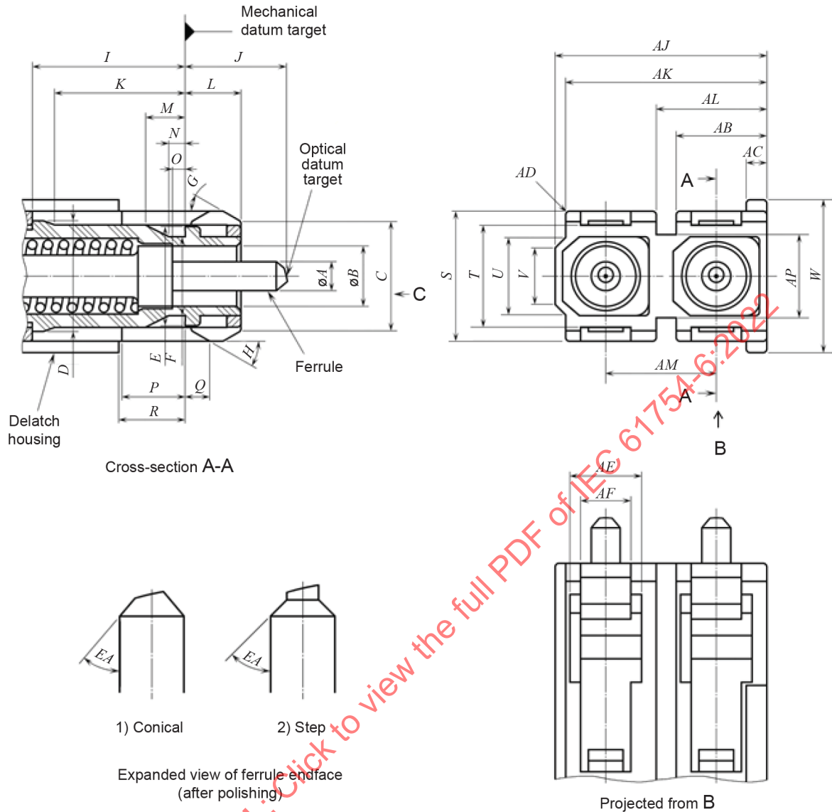
Figure 21 – 4,5 mm duplex plug connector interface – Push/pull, APC (1 of 2)
