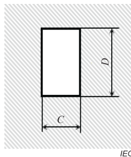
Figure D.2 – Panel cut out
