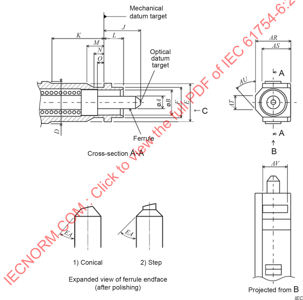
Figure 19 – Plug connector interface – For printed board housings, APC (1 of 2)
