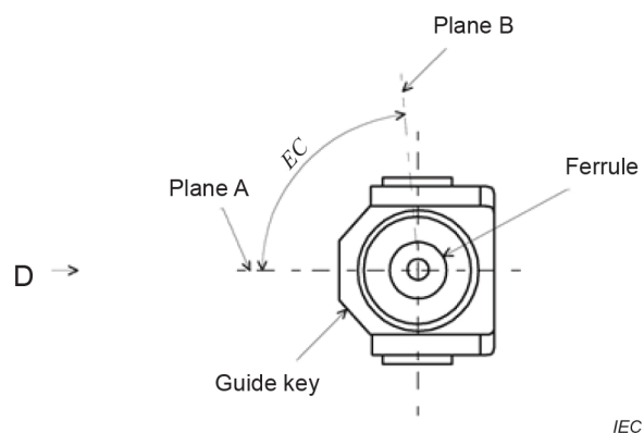
Expanded view from C direction (after polishing)
