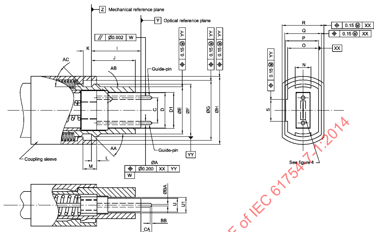
Figure 11 – MPO male plug, flat interface
