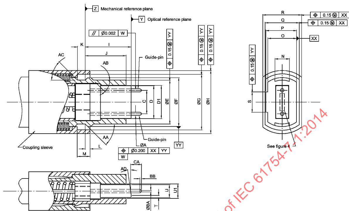
Figure 8 – MPO male plug, up-angled interface
