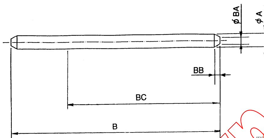
Figure 2c – Gauge pin
