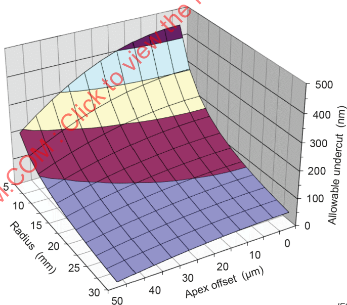
Figure A.1 – Allowable undercut as a function of endface radius and apex offset – 4,9 N minimum contact force
