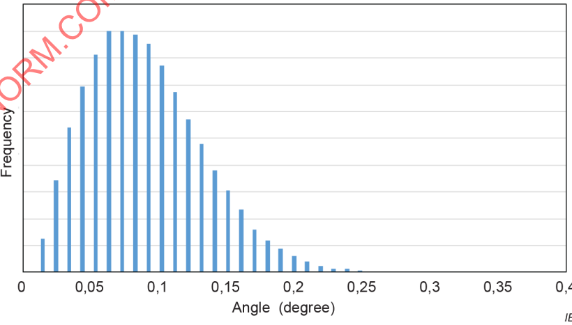
Figure C.3 – Resultant fibre angle distribution for Grade B attenuation
