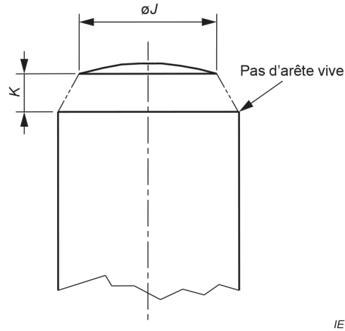
Figure 3 – Dimensions de la ferrule
