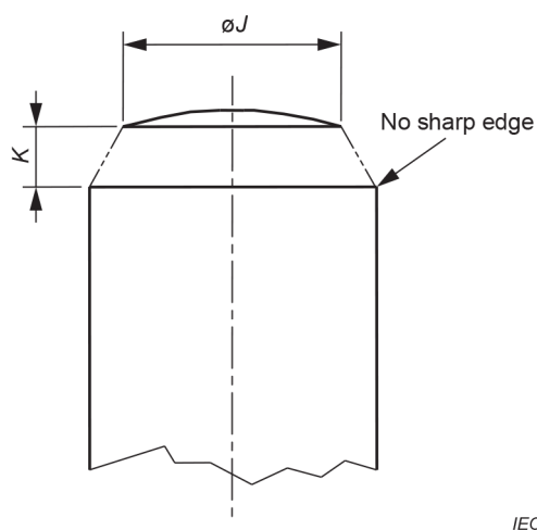
Figure 3 – Ferrule dimensions
