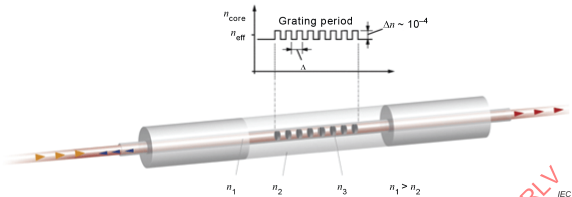
a) FBG refractive index profile and build-up
