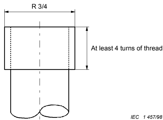
Figure 5 – Mandrel for testing coupling nuts
