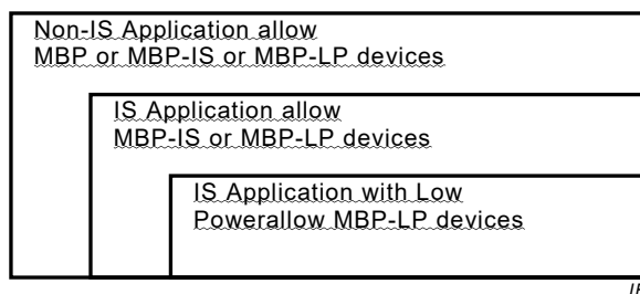
Figure 3 – CP 3/2 Slave devices usable in applications
