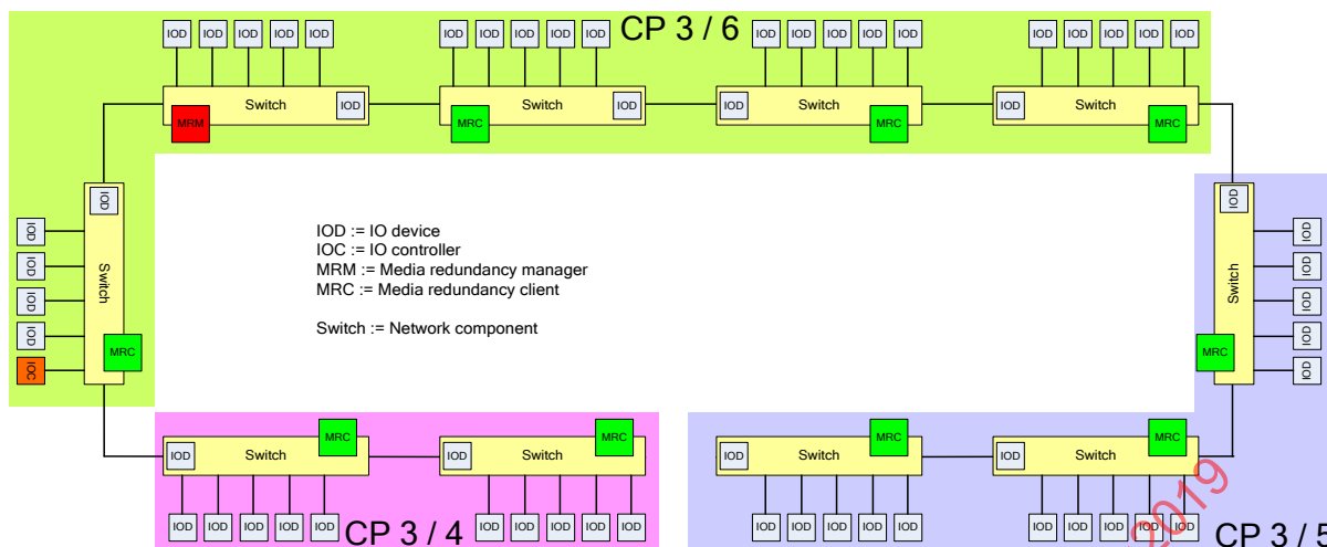
Figure 3 – Example of network topology using CP 3/4, CP 3/5, and CP 3/6 components
