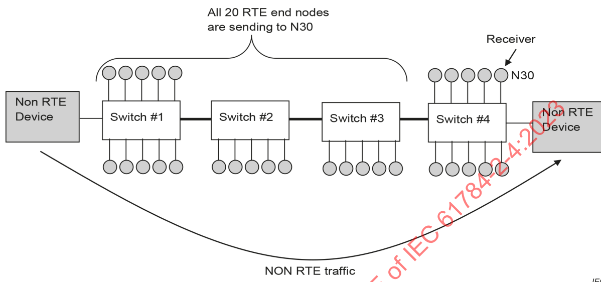
Figure A.2 – Non-RTE throughput calculation
