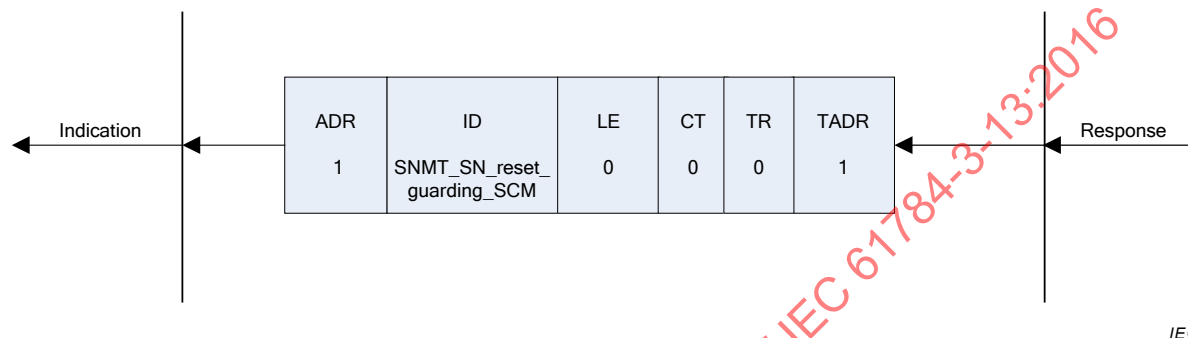
Figure 39 – Reset Node Guarding Time protocol
