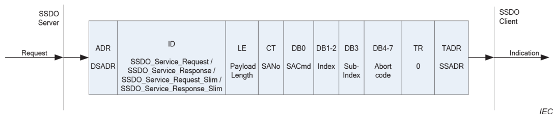
Figure 38 – SSDO Abort protocol
