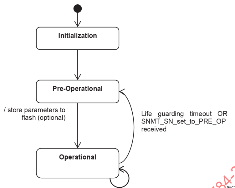
Figure 77 – State diagram SN power up
