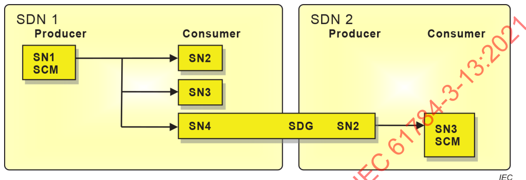
Figure 13 – Data flow example
