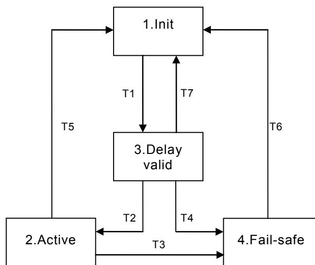
Figure 12 – RxSPDO state machine
