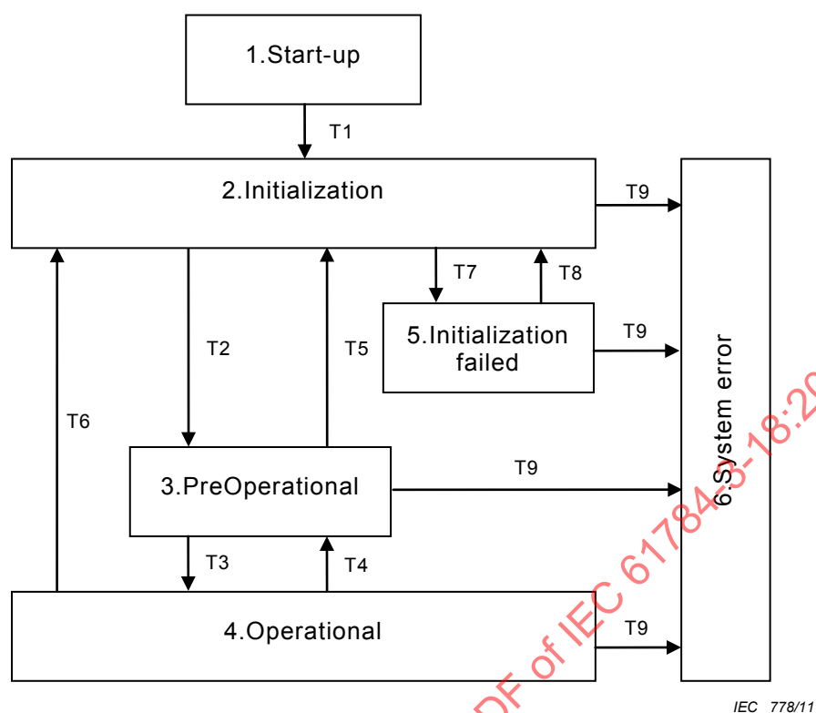
Figure 11 – SALMT state machine
