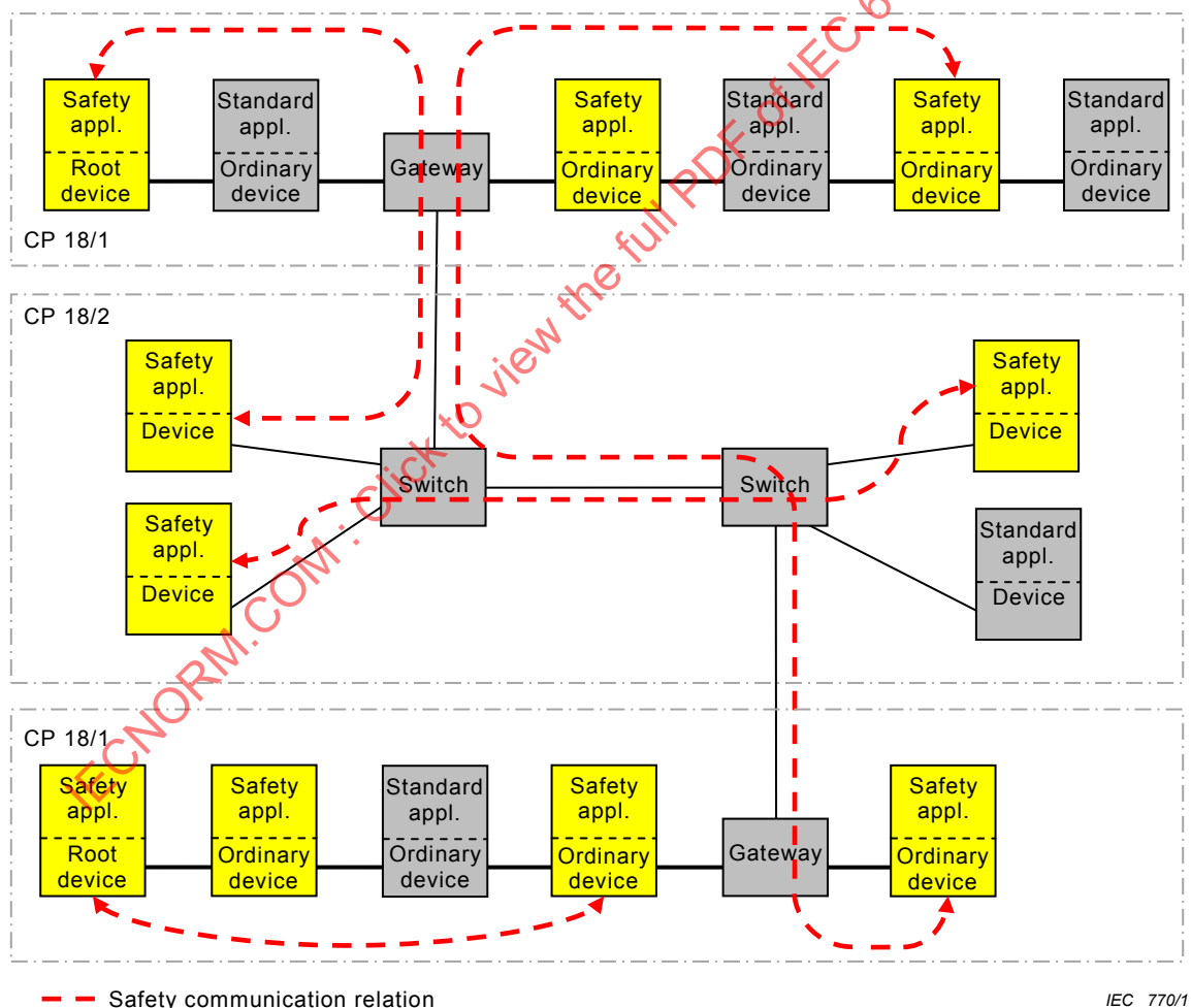
Figure 3 – FSCP 18/1 system
