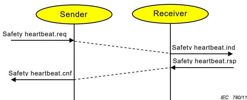
Figure 13 – Heartbeat procedure
