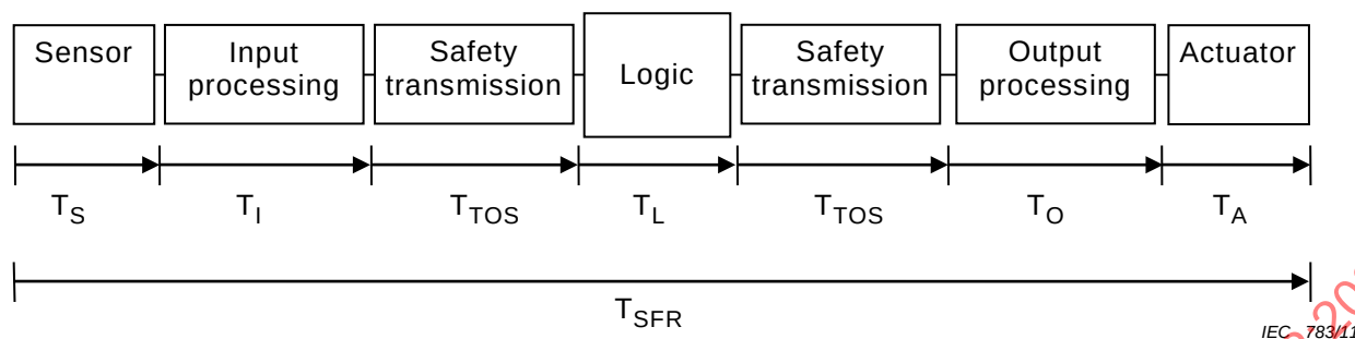
Figure 16 – Safety response time components
