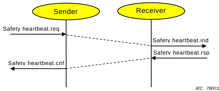
Figure 13 – Heartbeat procedure
