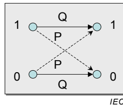
Figure B.2 – Binary symmetric channel (BSC)
