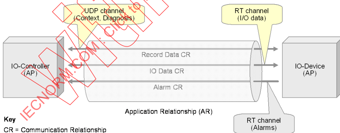
Figure 15 – Application and communication relationships (AR/CR)
