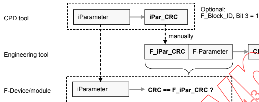
Figure 54 – CRC1 including iPar_CRC
