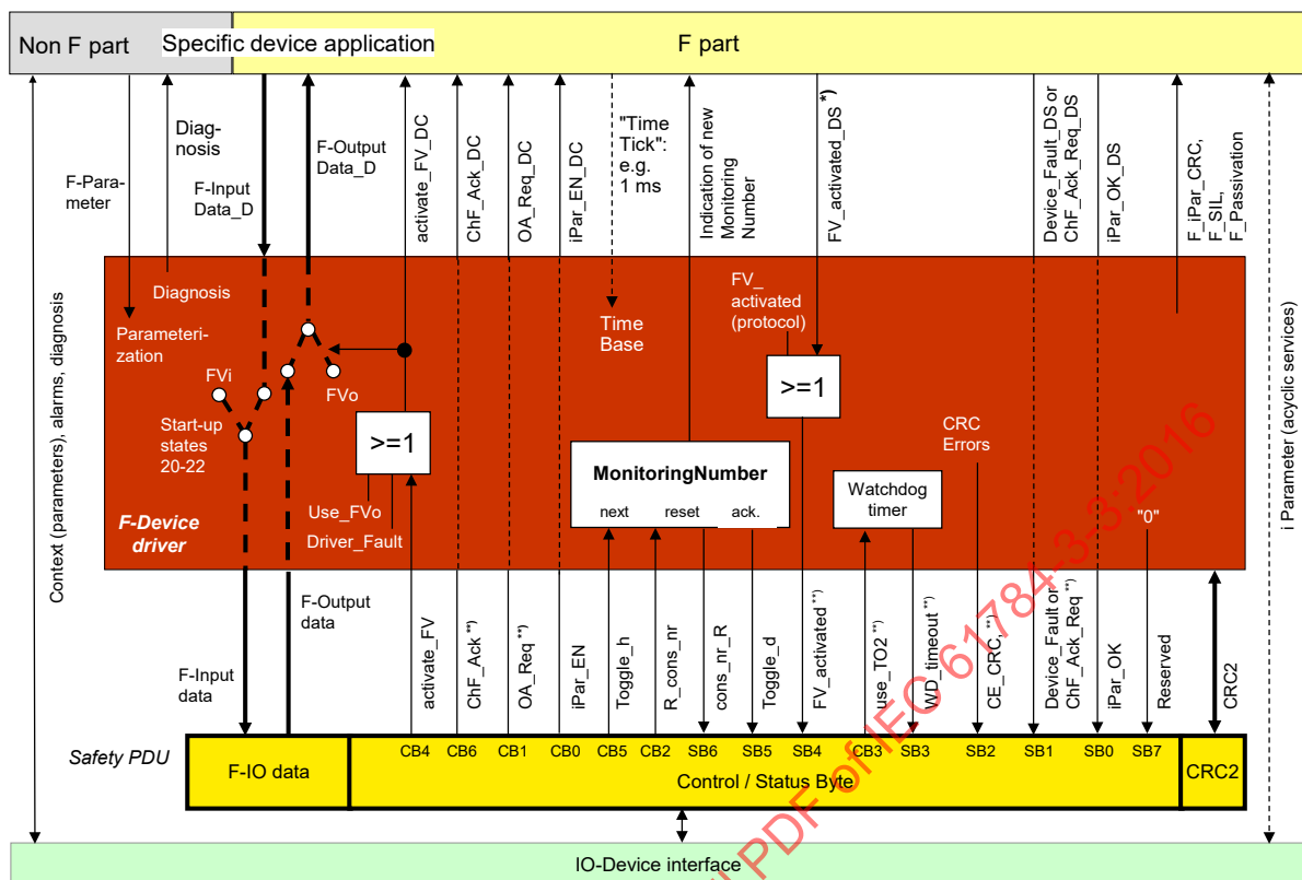
Figure 17 – F-Device driver interfaces
