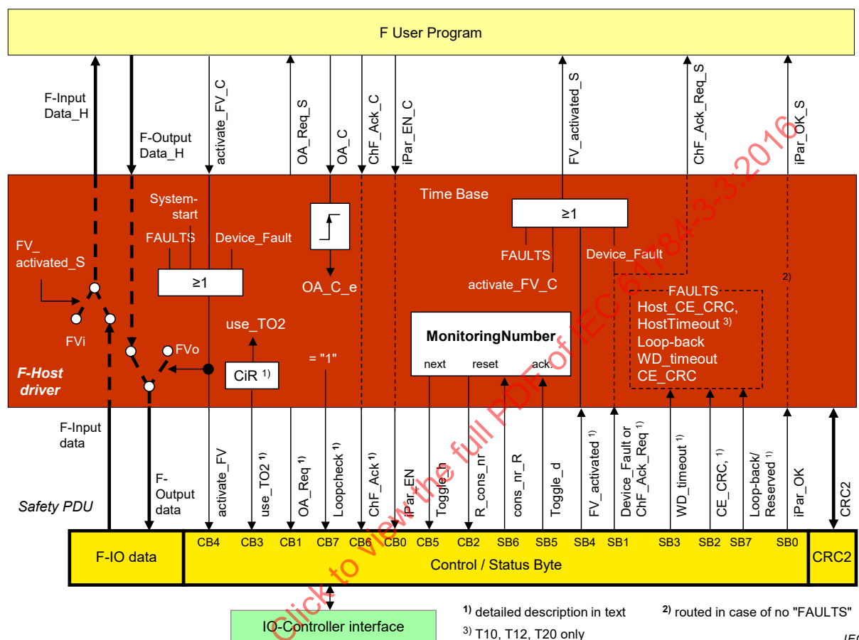
Figure 15 – F user interface of F-Host driver instances
