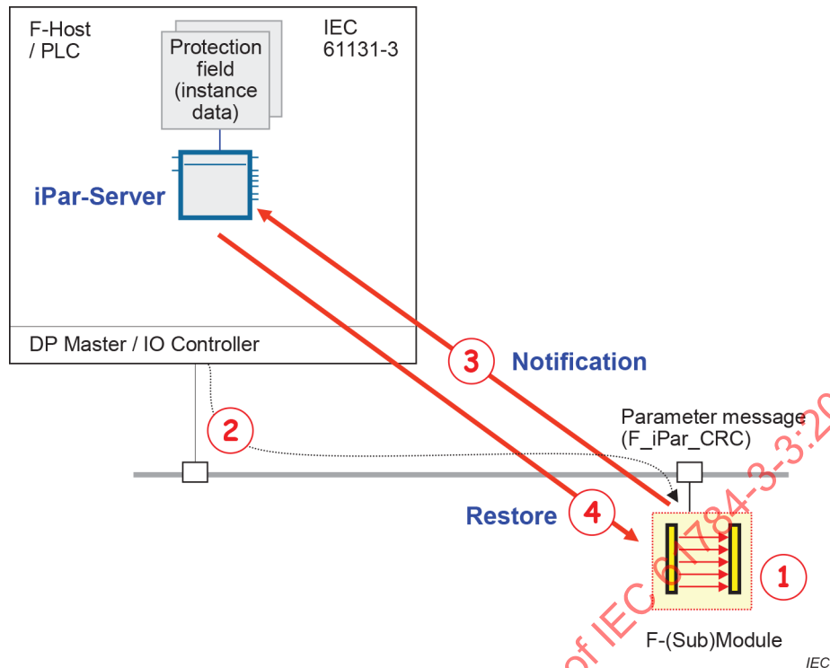
Figure 56 – iPar-Server mechanism (for example F-(Sub)Module replacement)
