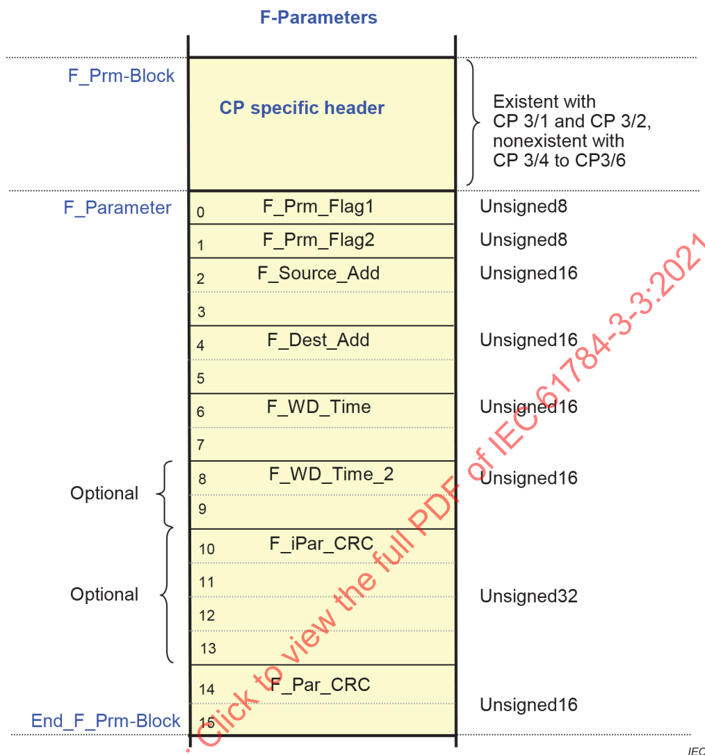
Figure 47 – F-Parameter
