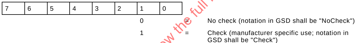
Figure 39 – F_Check_iPar
