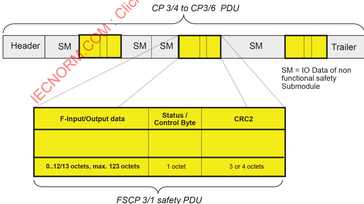
Figure 4 – Structure of an FSCP 3/1 safety PDU
