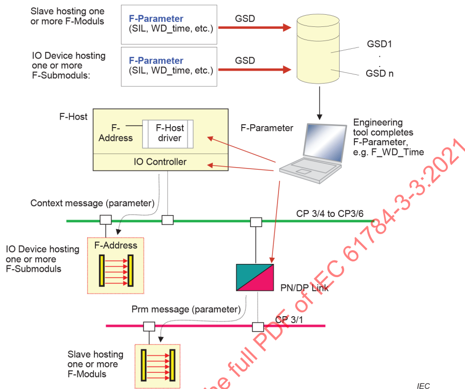
Figure 53 – F-Parameter assignment for F-(Sub)Modules
