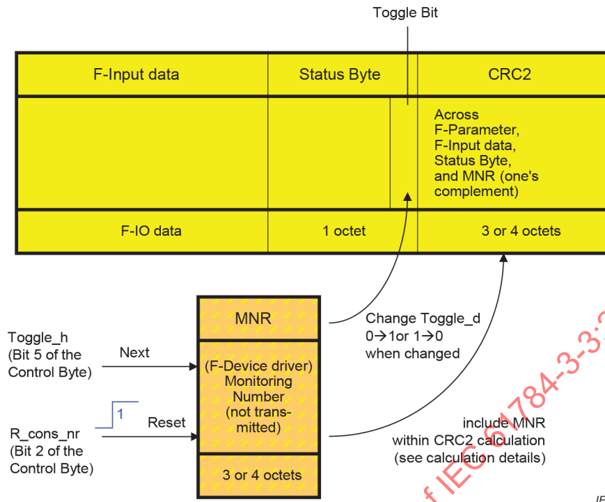
Figure 20 – MonitoringNumber integration
