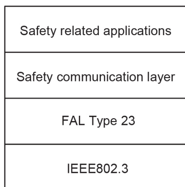
Figure 10 – Protocol Hierarchy
