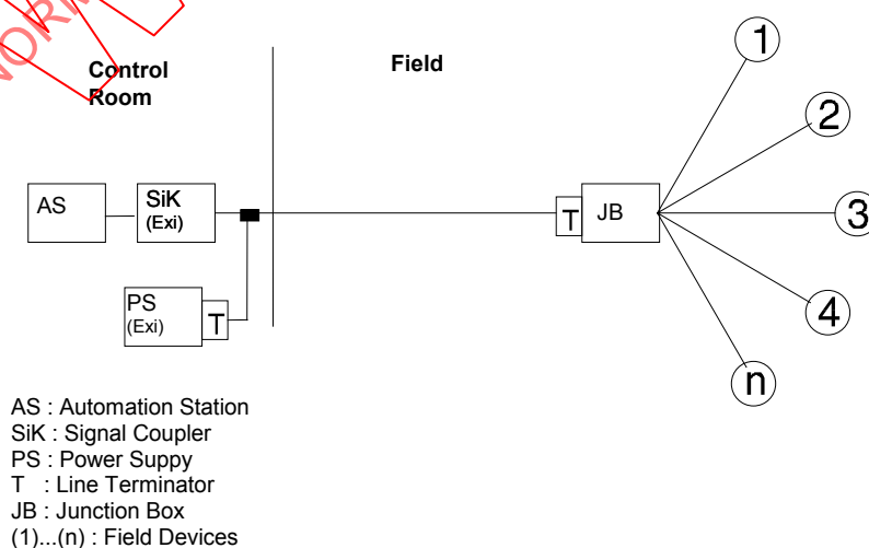
Figure B.6 – CP 3/2 topology
