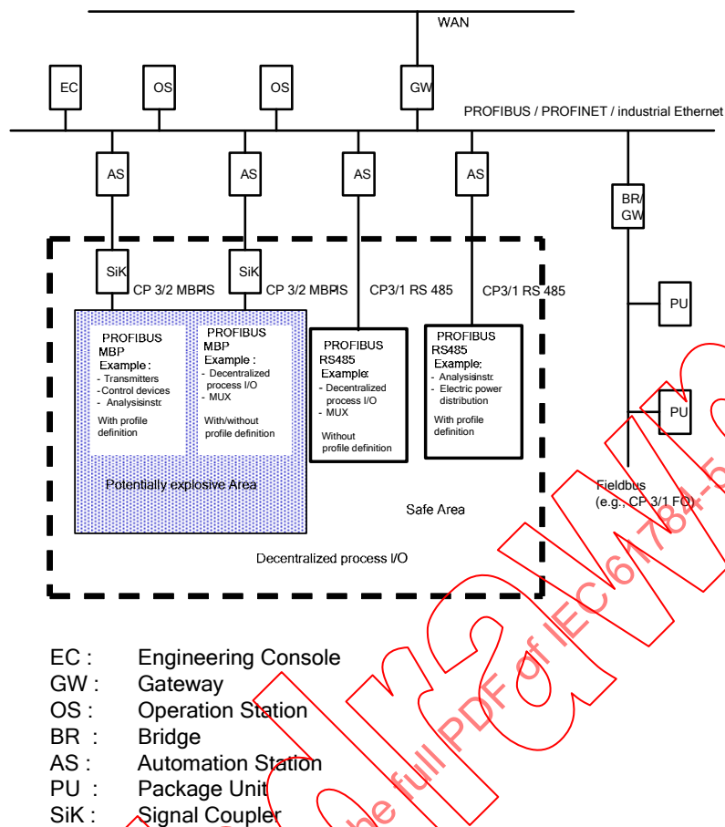
Figure B.1 – Connection of CP 3/1 networks
