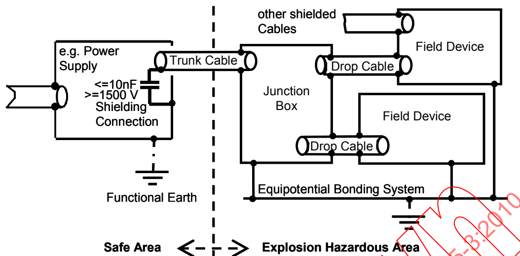
Figure B.12 – Capacitive earthing
