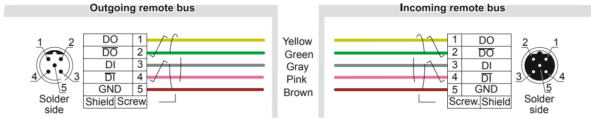
Figure A.5 – M12 circular connector pin assignments
